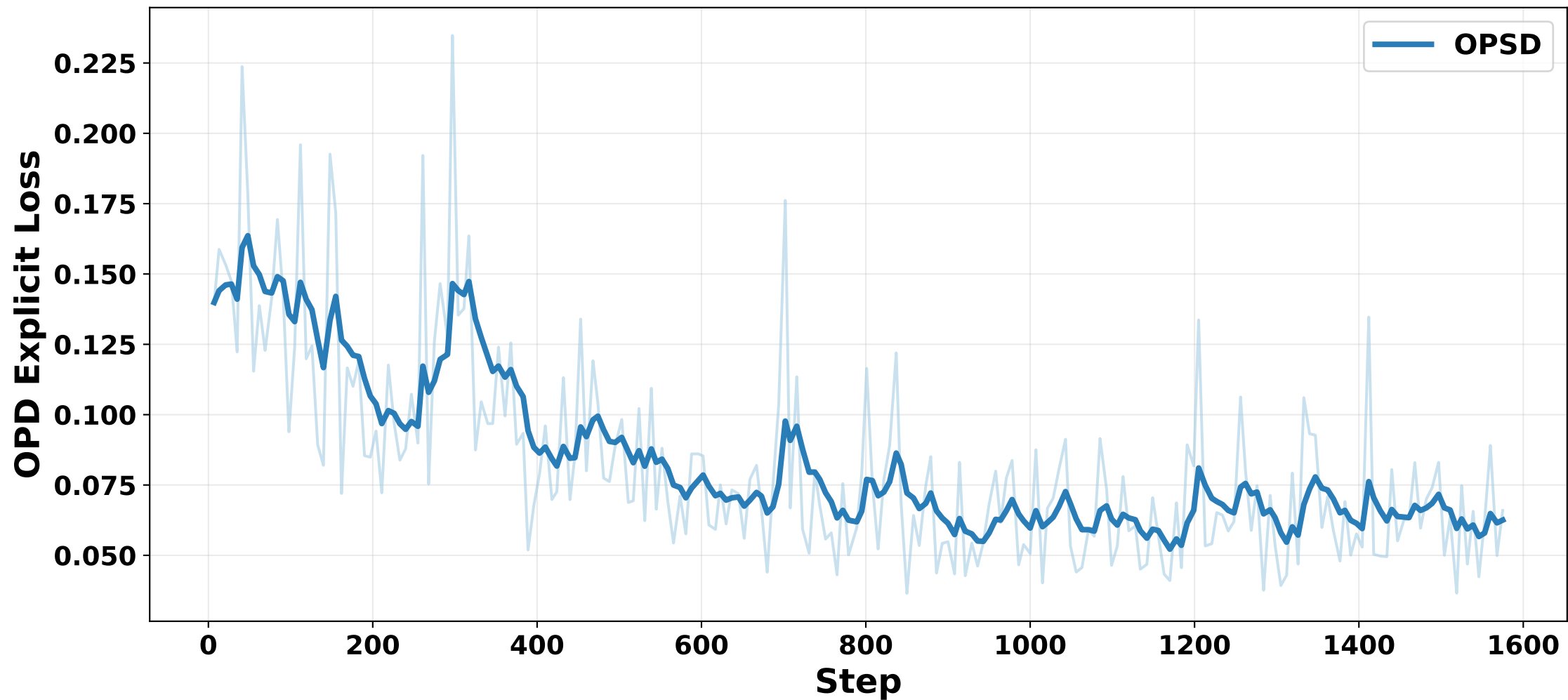
train/opd_explicit_loss
